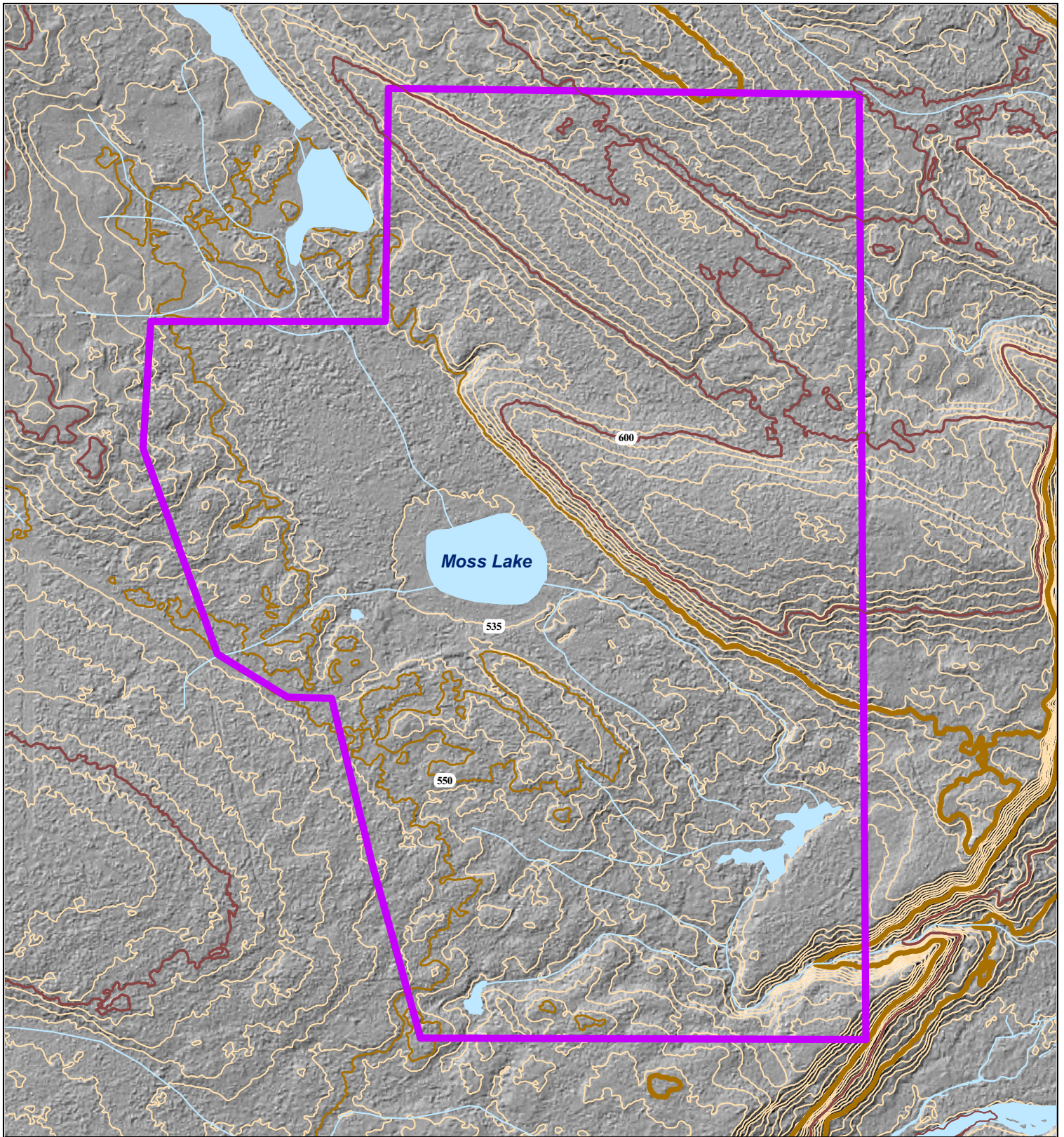
Moss Lake Natural Area Figure 4: Contours and Hillshade Map
